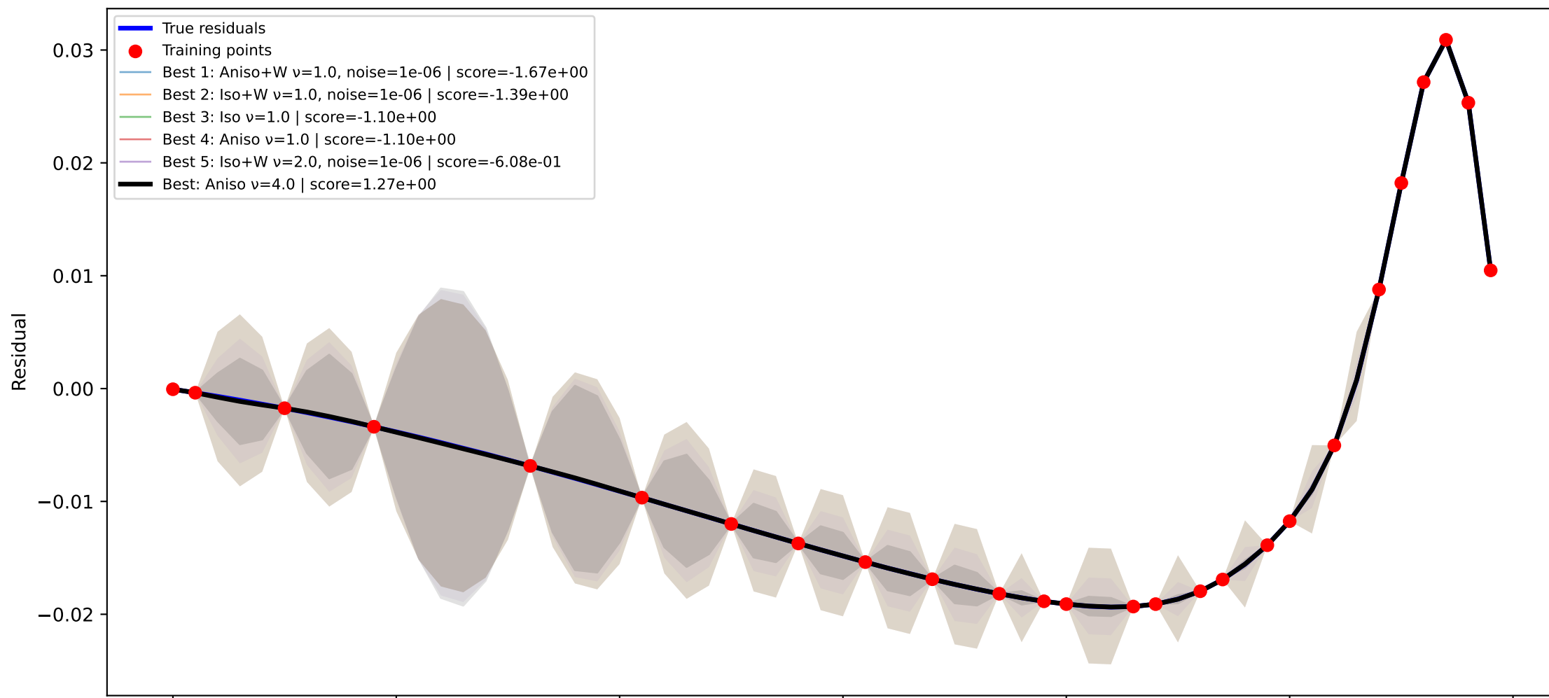
GPR kernel comparison node=9 RMSE=2.880e-05, train RMSE=1.811e-11
